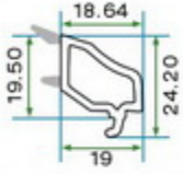
K 6006 DEKORATİF ÇİFT CAM ÇİTASI K 6006 DECORATIVE DOUBLE GLAZING BEAD WITH GRAY GASKET
