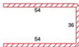
KAPI KANAT DESTEK SAÇI DOOR SASH STEEL REINFORCEMENT
