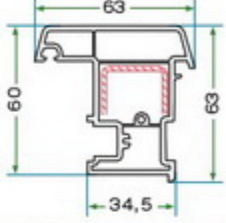
K 6021 HAREKETLİ ORTA KAYIT PROFİLİ K 6021 MOVABLE MULLION PROFILE
