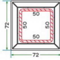
KKS 6007 70 mm KUTU PROFİL KKS 6004 70 mm BOX PROFILE
