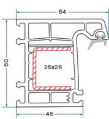
K 6001 KASA PROFİLİ K 6001 FRAME PROFILE
