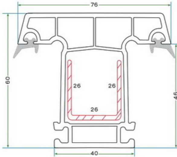
KYS 8002 ORTA KAYIT PROFİLİ KYS 8002 MULLION PROFILE
