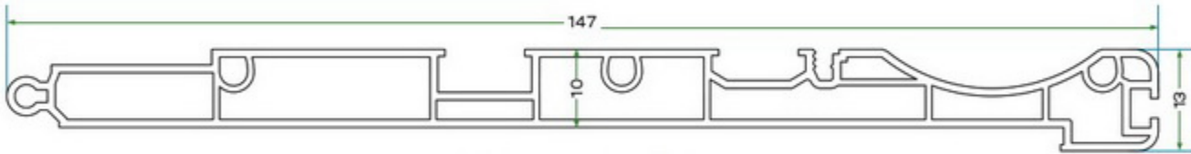
KMS 006 PANJUR ALT PROFİL KMS 006 PANJUR ALT PROFİL
