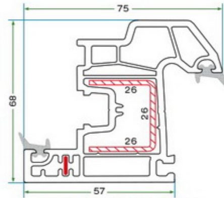
K 6003 DAMLALIKLI KANAT PROFİLİ K 6003 DROPPER SASH PROFILE
