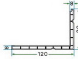
K 6010 80x120 PERVAZ PROFİLİ K 6010 80 x 120 BORDER PROFILE
