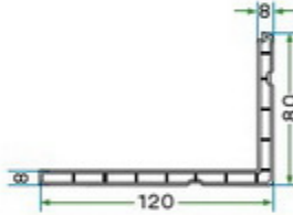
K 6010 80 x 120 PERVAZLI PROFİLİ K 6010 80 x 120 BORDER PROFILE
