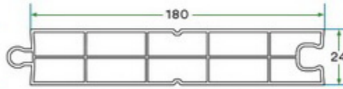
K 6032 LAMBİRİ PROFİLİ K 6032 PANEL PROFILE
