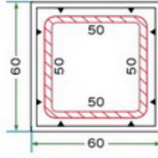
KKS 6009 60 x 60 KUTU PROFİLİ KKS 6009 60 x 60 BOX PROFILE
