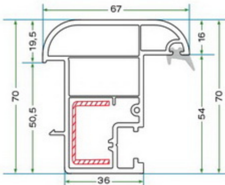
KRS 009 70'LİK OVAL HAREKETLİ ORTA KAYIT PROFİLİ KRS 009 OVAL MOVABLE MULLION PROFILE
