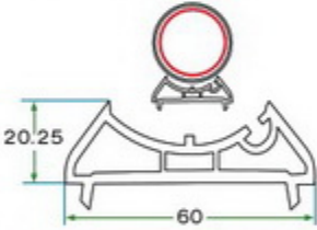
KKS 6011 60 mm DÖNÜŞ ADAPTÖRÜ KKS 6011 60 mm CORNER ADAPTER
