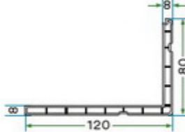
K 6010 80 x 120 PERVAZLI PROFİLİ K 6010 80 x 120 BORDER PROFILE
