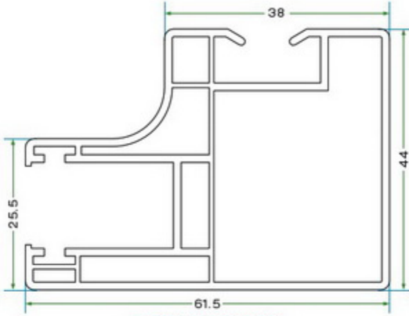
KMS 004 PANJUR YAN DİKME KMS 004 PANJUR YAN DİKME
