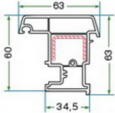
K 6021 HAR. ORTA KAYIT PROFİLİ K 6021 MOVABLE MULLION PROFILE
