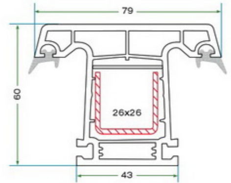
K 6002 ORTA KAYIT PROFİLİ K 6002 MULLION PROFILE
