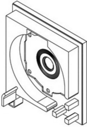
PANJUR 5'li KUTU KAPAK SETİ (SAĞ) SHUTTER 5-PIECE BOX COVER SET (RIGHT)
