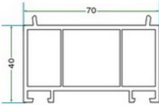
KRS 011 KASA YÜKSELTME APARATI KRS 011 CASE UPGRADE APPARATUS
