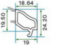
K 6006 DEKORATİF ÇİFT CAM ÇİTASI K 6006 DECORATIVE DOUBLE GLAZING BEAD WITH GRAY GASKET
