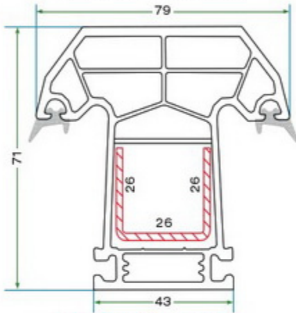
KKS 002 ORTA KAYIT PROFİLİ KKS 002 MULLION PROFILE
