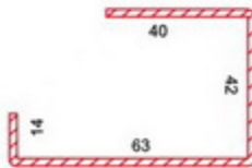
KAPI DESTEK SAÇI FOR DOOR SASH STEEL REINFORCEMENT
