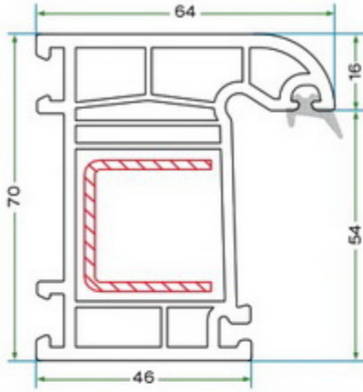
KRS 001 70'LİK KASA PROFİLİ KRS 001 70 FRAME PROFILE
