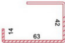
KAPI DESTEK SAÇI DOOR STEEL REINFORCEMENT
