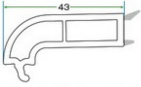
KRS 006 70'LİK TEK CAM ÇİTASI KRS 006 70 SINGLE GLASS BEAD WITH GRAY GASKET
