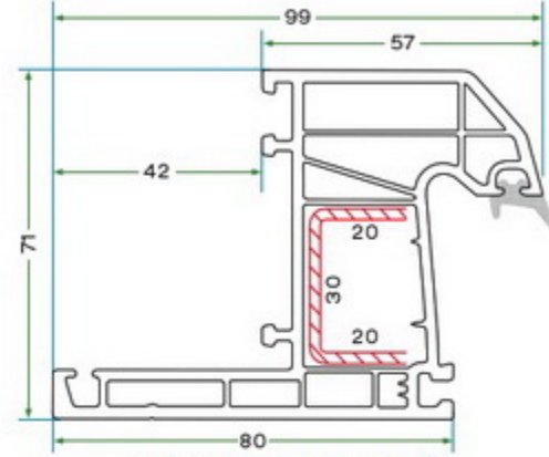
KKS 007 PERVAZLI KASA PROFİLİ KKS 007 FRAME PROFILE WITH BORDER
