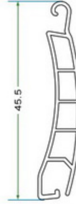
KMS 005 LAMEL KMS 005 LAMEL
