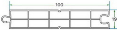
K 6008 LAMBİRİ PROFİLİ K 6008 PANEL PROFILE
