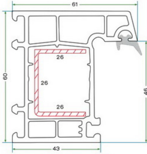
KYS 8001 KASA PROFİLİ KYS 8001 FRAME PROFILE
